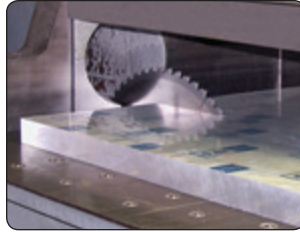
Plate Sawing
