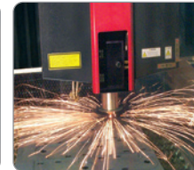
Plate Laser Cutting
