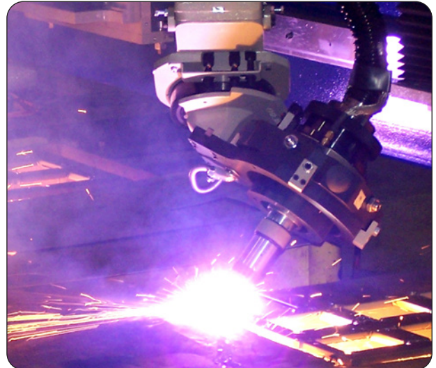
Plasma cutting machine with bevel cutting capabilities.
